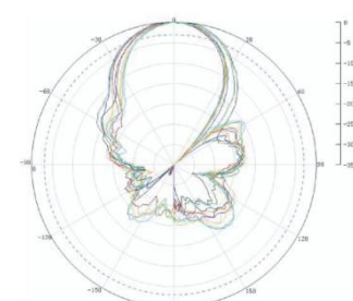
Vertical Elevation
